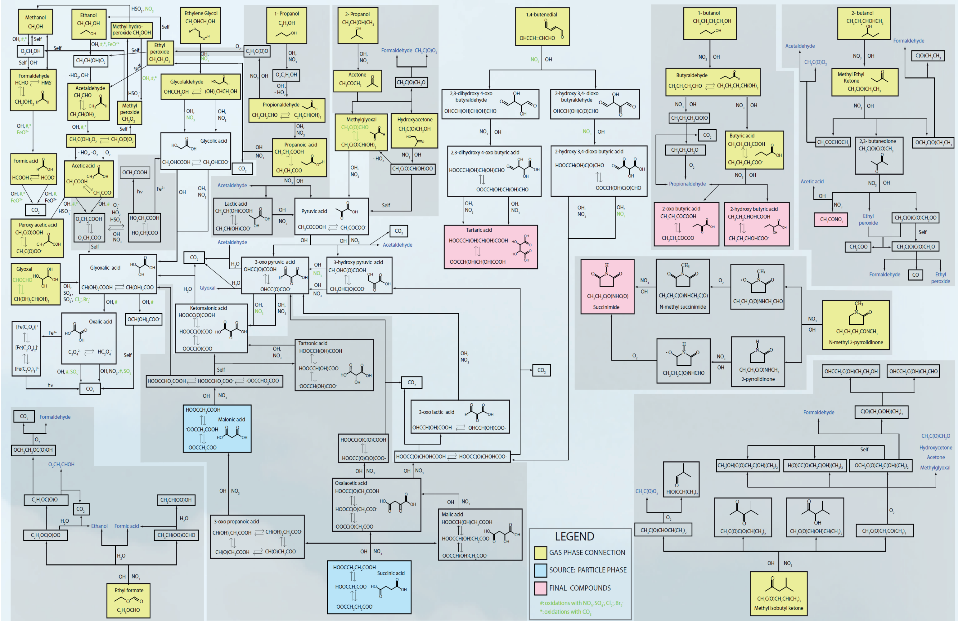
Schematic depiction of the organic chemistry in C3.0RED. The reduced chemical organic subsystems compared to the full CAPRAM 3.0i mechanism are indicated by a grey background and marked in green. (For purpose of clarity, the explicit oxidation scheme of the full aqueous phase mechanism including peroxy radical formation and recombination reactions is not displayed as far as these processes are not considered in the reduced mechanism.)
